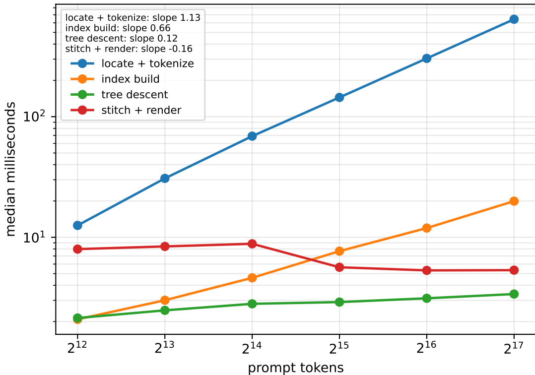
Compiler cost per stage (log-log slope = exponent in n )
