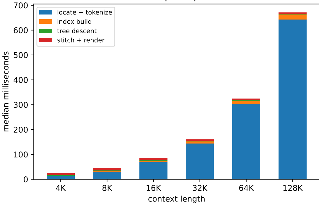
Where the compiler spends its time
