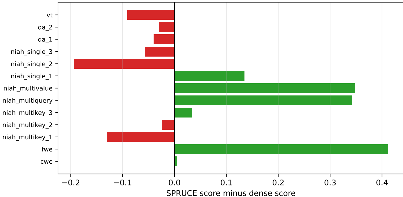
Per-task delta (green favours SPRUCE)
