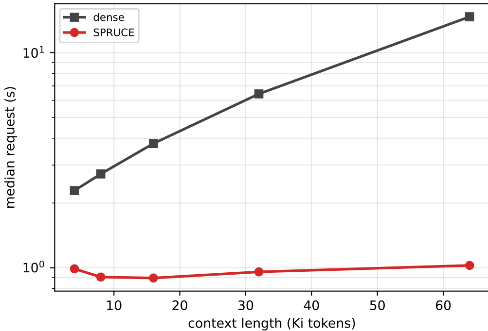
Fully charged request cost on RULER
