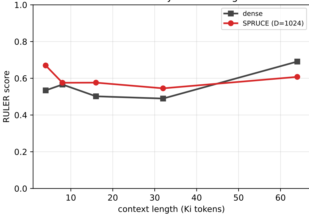
RULER score by context length
