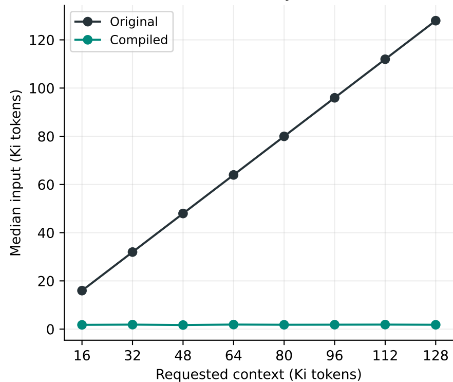
Tokens read by Qwen
