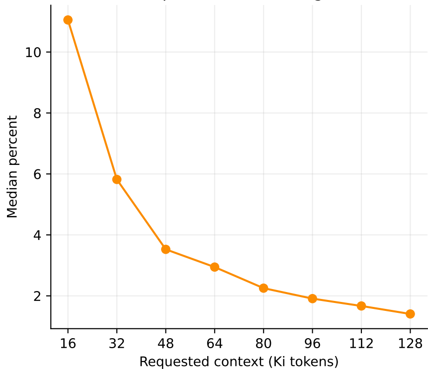
Compiled fraction of original
