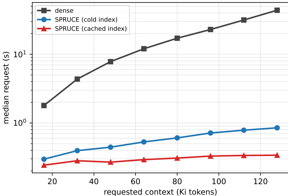
Fully charged request cost
