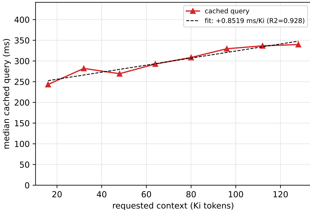
Cached per-query latency against context length
