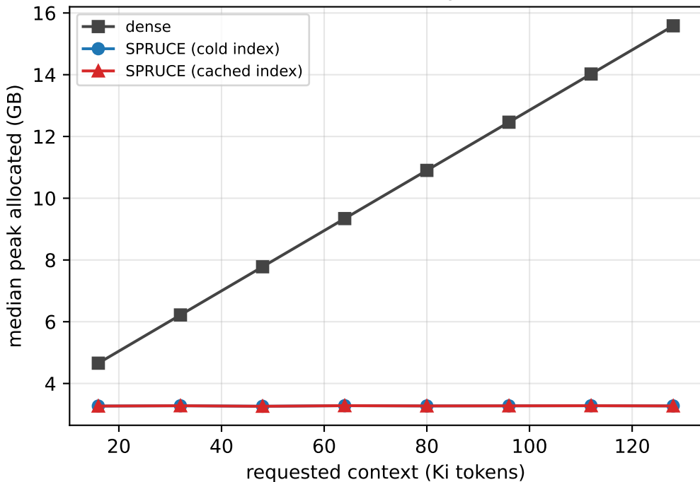
GPU memory
