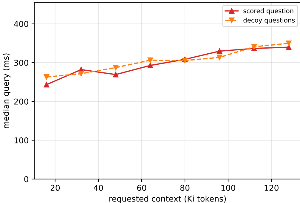
Cached cost does not depend on the question
