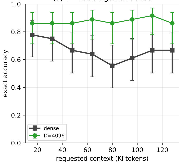
(a) D=4096 against dense
