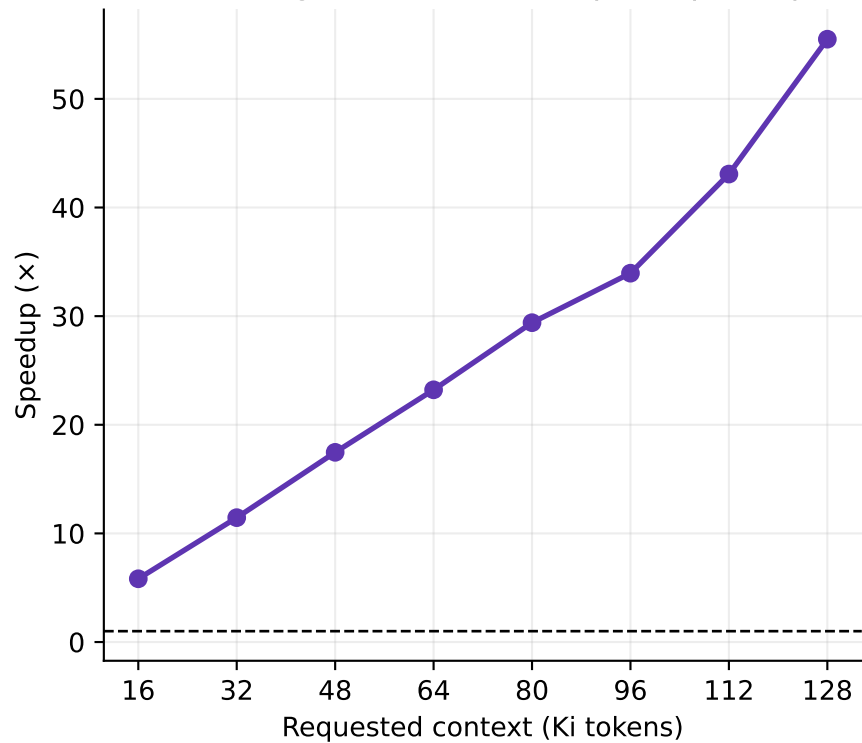
Sum-weighted dense / compiler speedup
