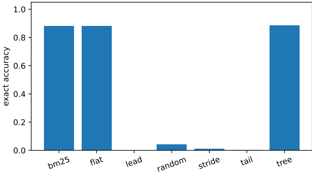
Generated accuracy at a matched block budget (L4)
