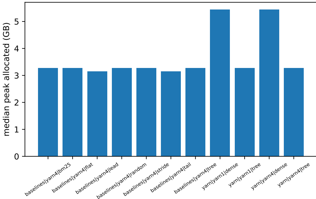
Peak allocated GPU memory per arm (L4)
