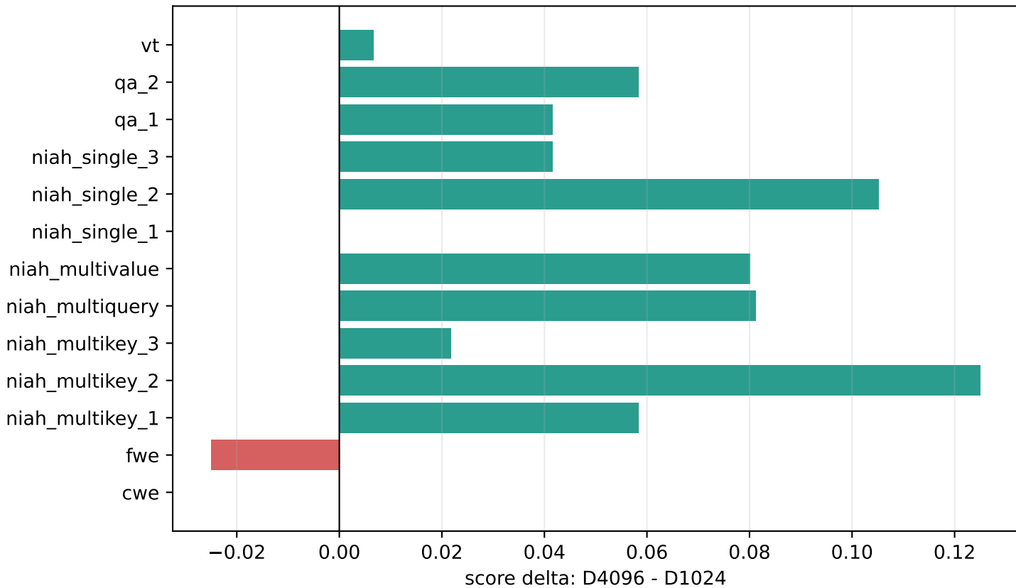
Paired feature-width effect by task
