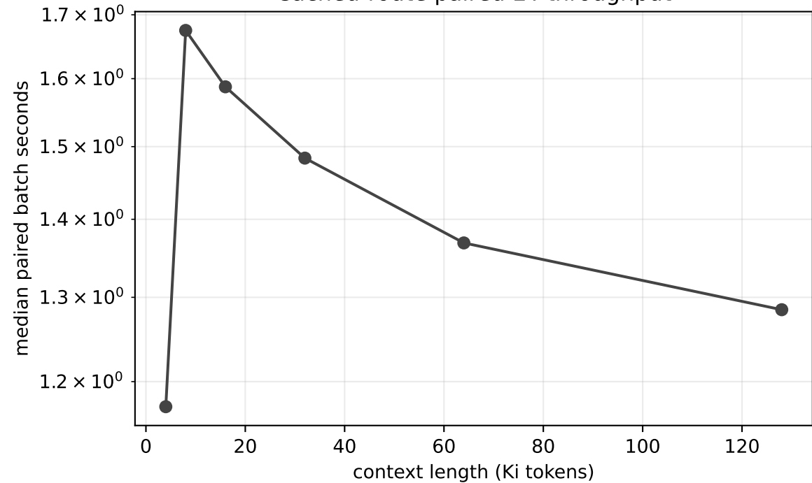
Cached-route paired L4 throughput
