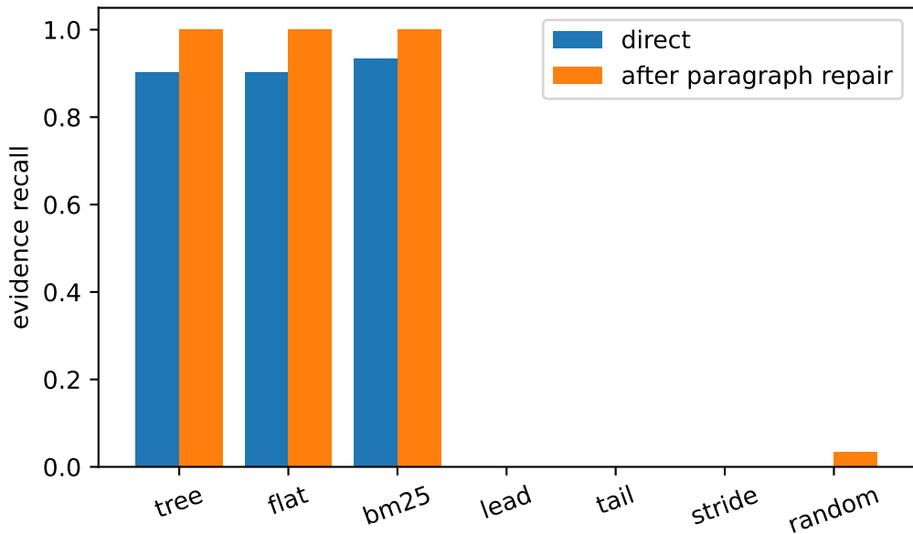
Evidence recall at a matched block budget
