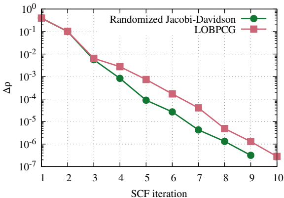
Si — Density convergence
