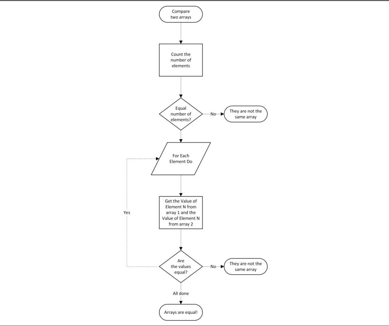
Figure J.1 — Comparing two arrays
