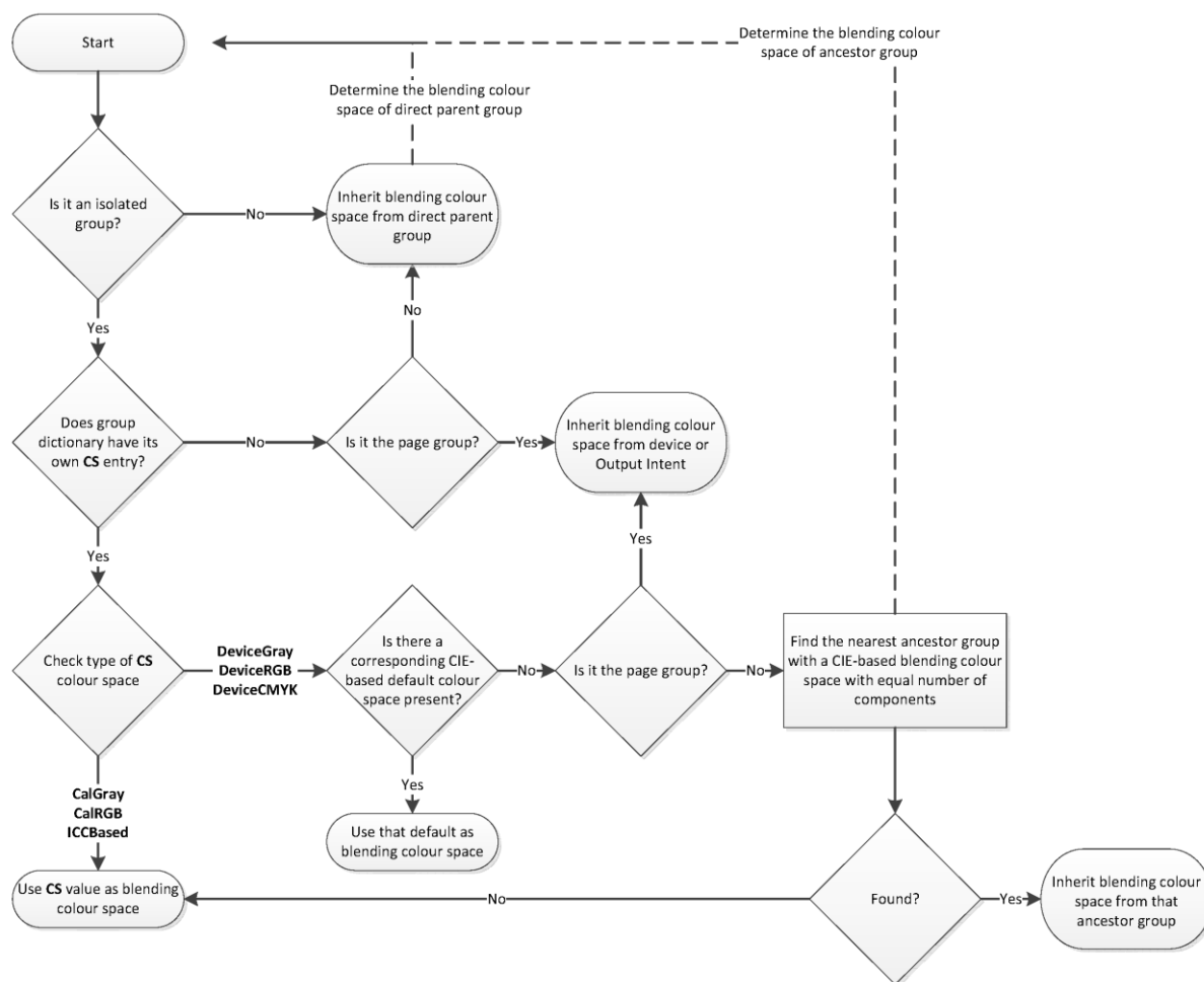
Figure P.1 — A possible algorithm to determine the blending colour space of a transparency group
