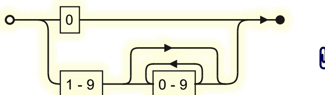
Figure 1d - EBNF diagram for a PDF generation number
