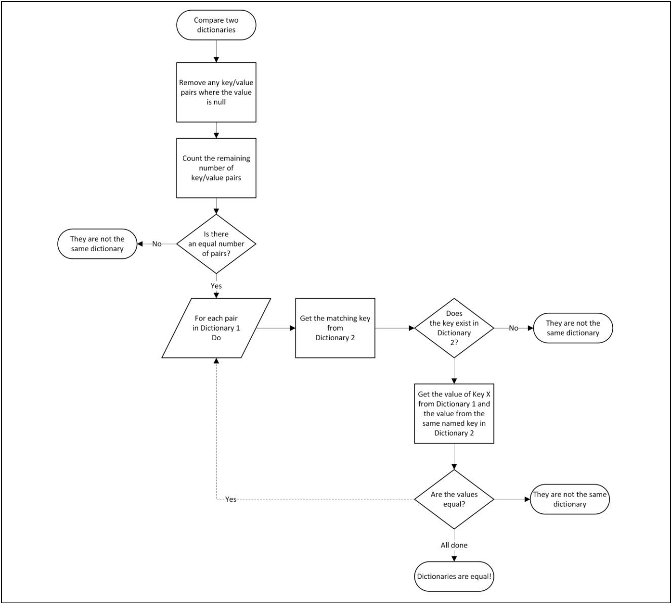
Figure J.2 — Comparison of two dictionaries
