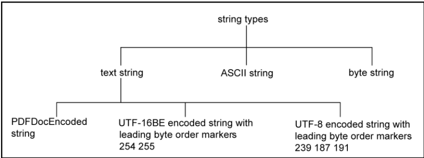
Figure 7 — Relationship between string types
