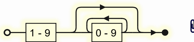
Figure 1c - EBNF diagram for a PDF object number
