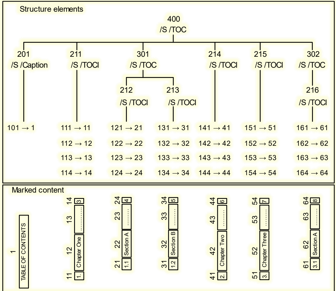
Figure H.7 — Hierarchy of structure elements and relationship with marked-content
