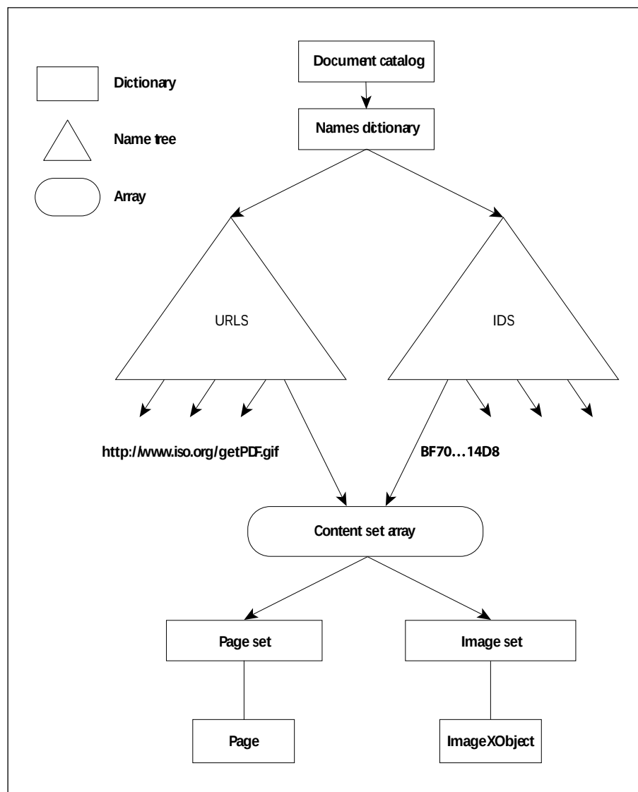
Figure 115 — Complex Web Capture file structure
