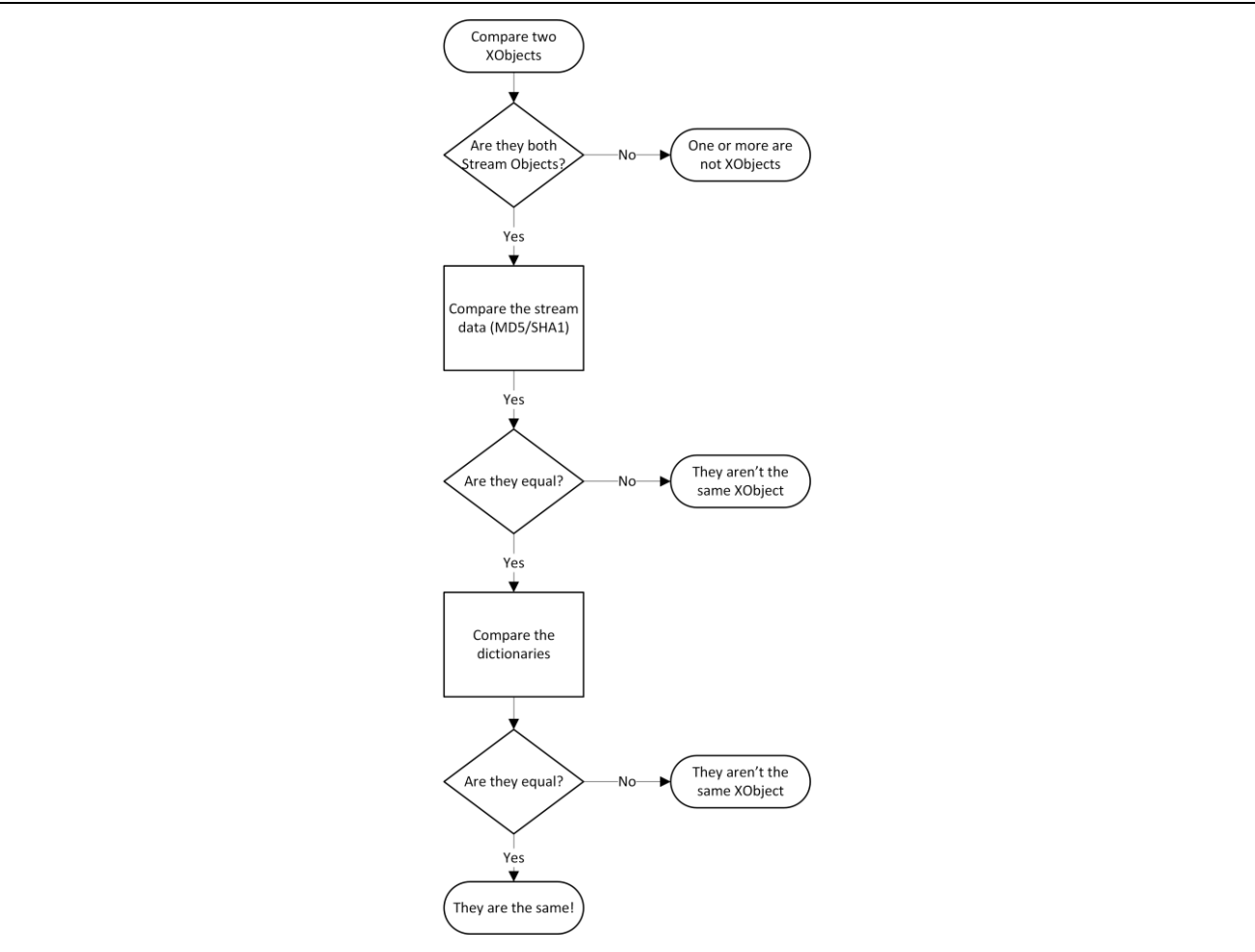
Figure J.3 – Comparing two XObjects
