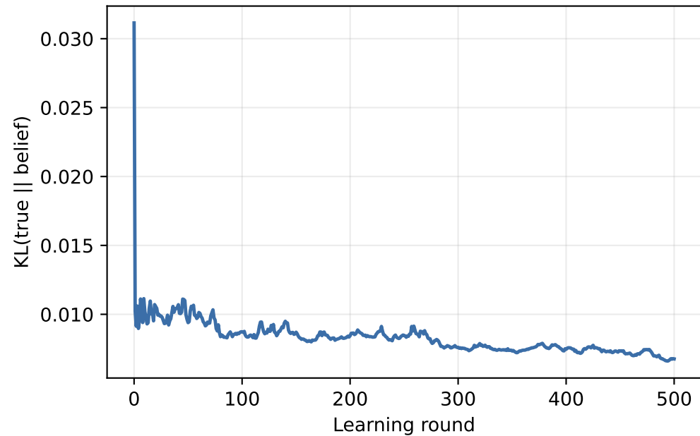
Prior-learning convergence
