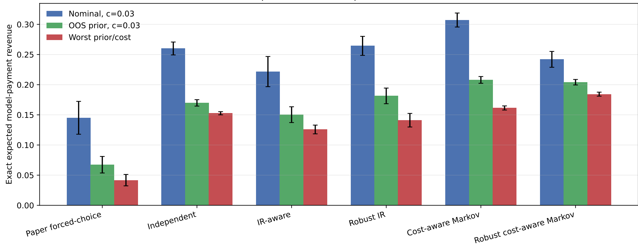
Mechanism improvements across perturbed market instances
