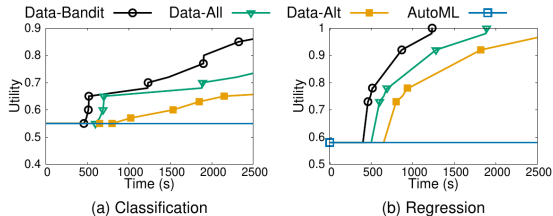
Figure 3: Compare discovery techniques on 1K input tasks.
