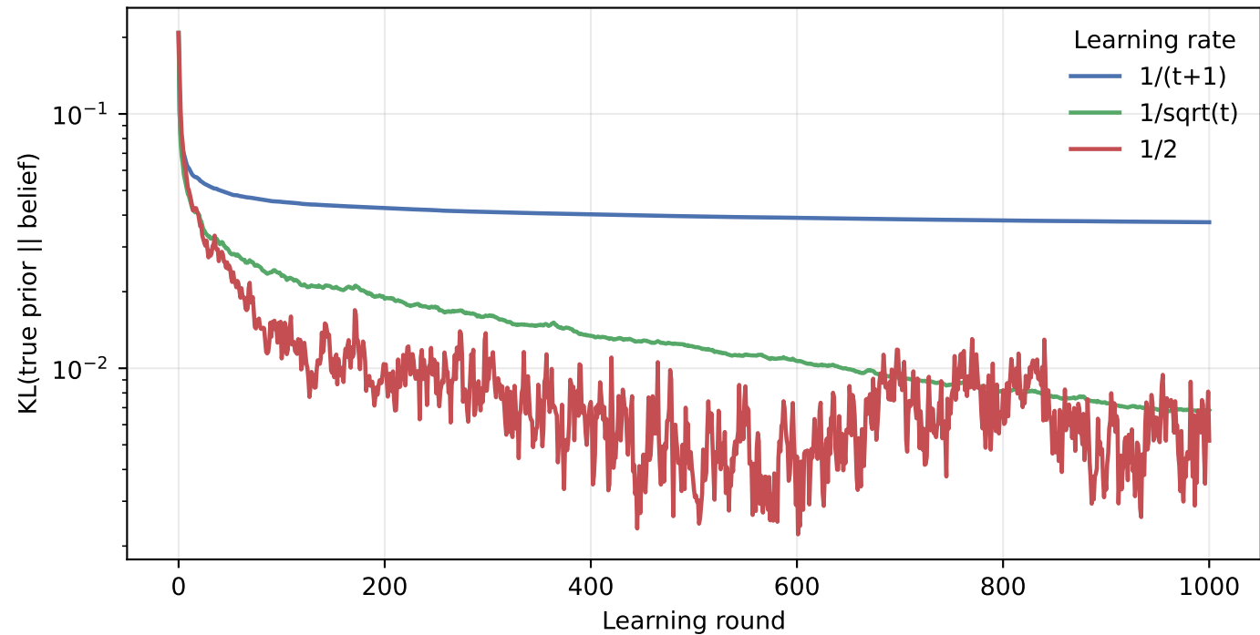
RQ3 reduced reproduction: random prior, batch size 100
