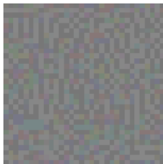
perturbation ( \times 8 )
