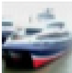
adversarial: "car" ✗
