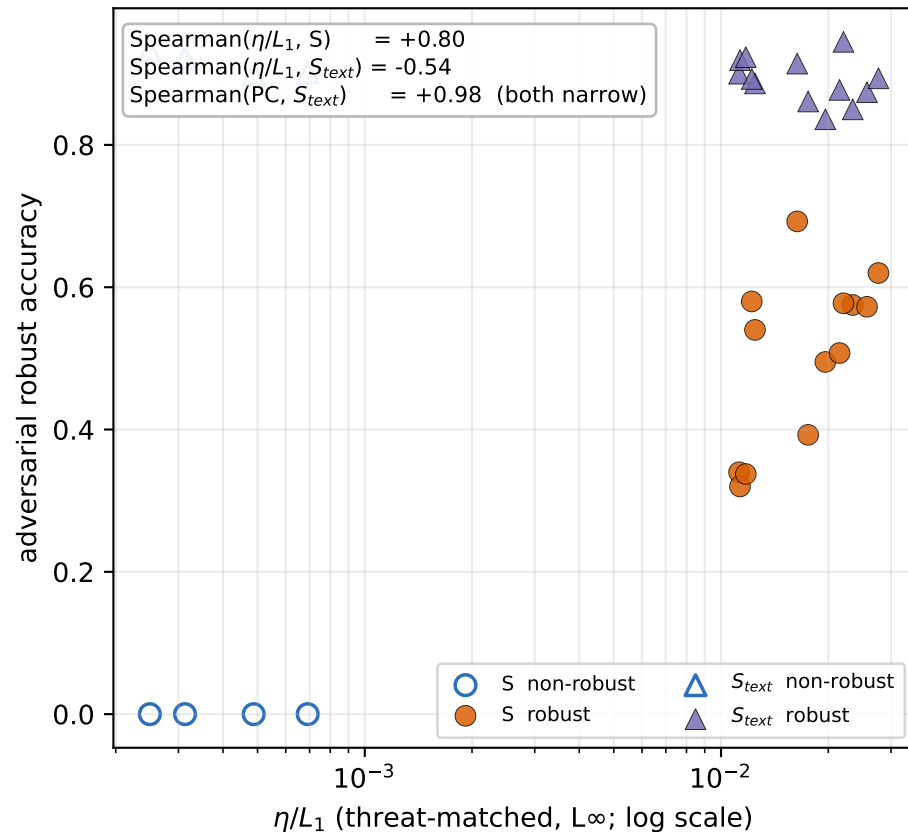
B. \eta/L_1 predicts the image cell (S), not the text cell ( S_{text} ); the consistencies predict neither
