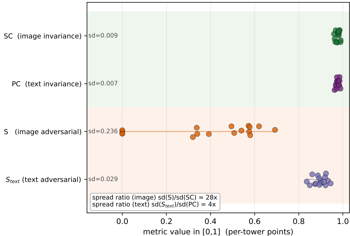
A. Both invariance cells saturate; the image-adversarial cell (S) spreads wide, the text cell ( S_{text} ) stays narrow
