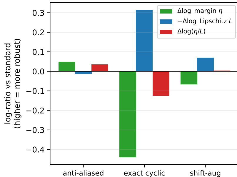
width 32 (AT)
