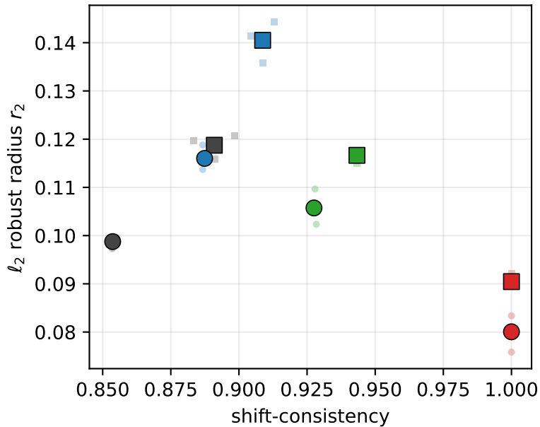
Pearson -0.55, Spearman -0.42
