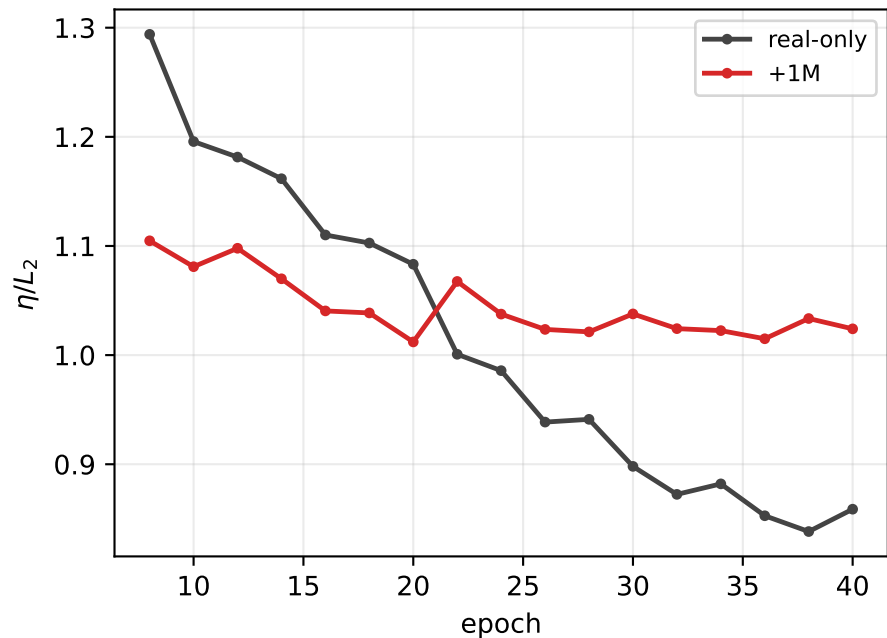
Robust overfitting = \eta/L collapse (baseline falls late; +1M holds)
