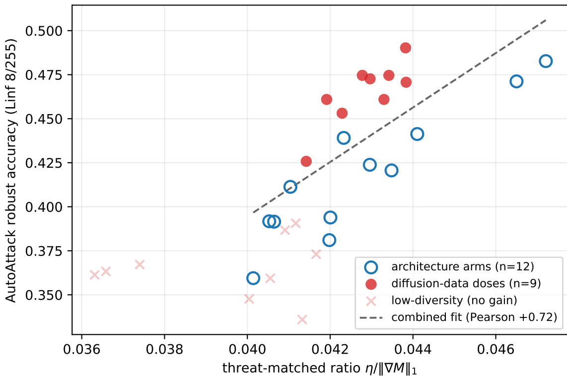
One law across interventions: architecture and data (same CIFAR-10 Linf-8/255 PreActResNet-18 AT setup)
