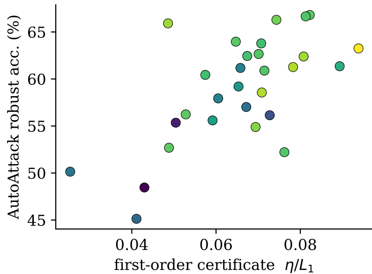
(b) size detects, ranks weakly Spearman = +0.57
