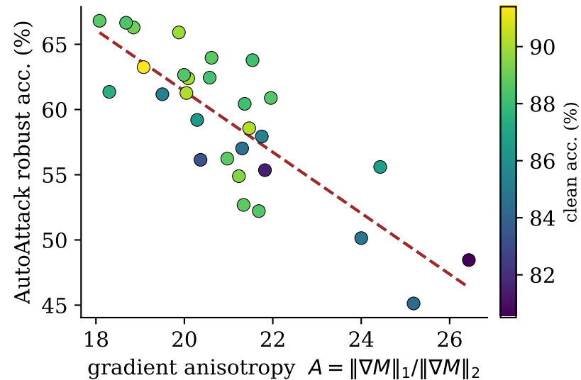
(a) shape ranks robust models Spearman = -0.77 ( p = 1e-06 )
