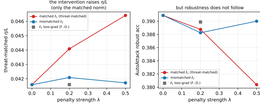
Figure 8: Regularizing \eta/L during adversarial training (standard backbone; means over widths and seeds). Left: only the threat-matched \ell_1 margin penalty raises \eta/L as its strength \lambda grows; the mismatched \ell_2 margin penalty and the \ell_2 loss-gradient penalty leave it flat. Right: the higher \eta/L does not raise AutoAttack robust accuracy, which is flat and then falls. Raising \eta/L by penalizing the gradient also shrinks the margin (the self-limiting coupling), so \eta/L is a diagnostic, not a training target.
