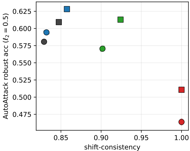
Pearson -0.81, Spearman -0.44
