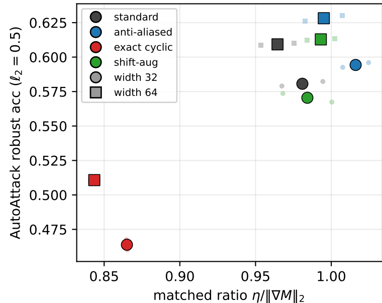
Pearson +0.88, Spearman +0.69
