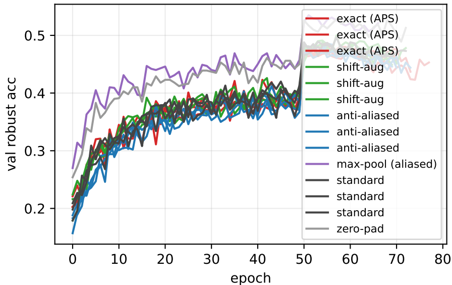
AT trajectories (robust overfitting)
