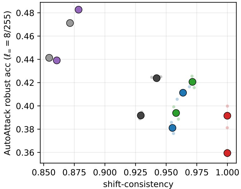
Pearson -0.81
