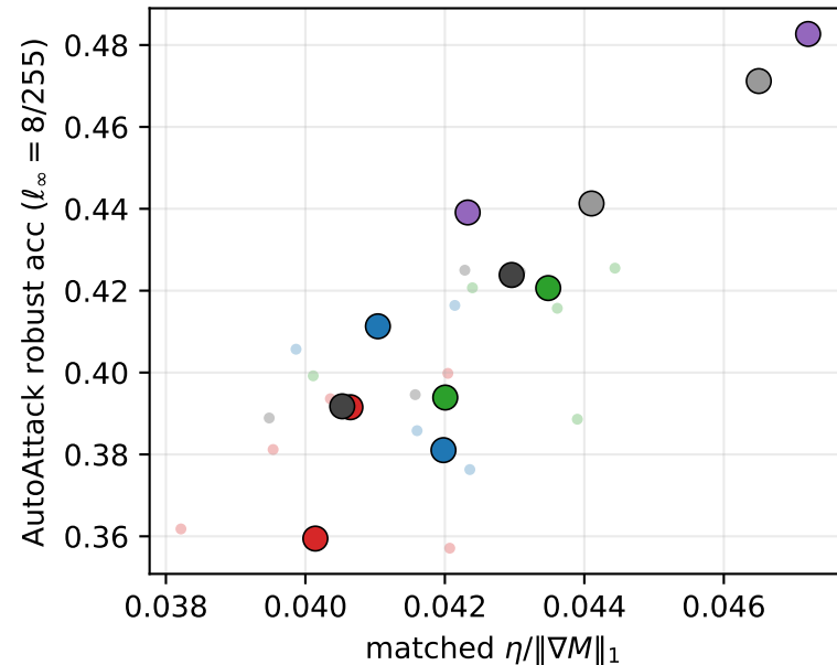
Pearson +0.91
