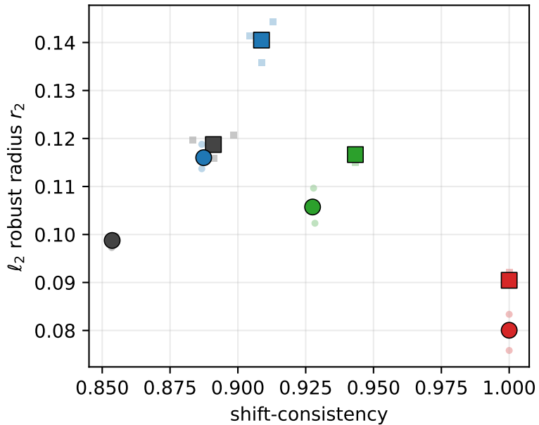
Pearson -0.55, Spearman -0.42
