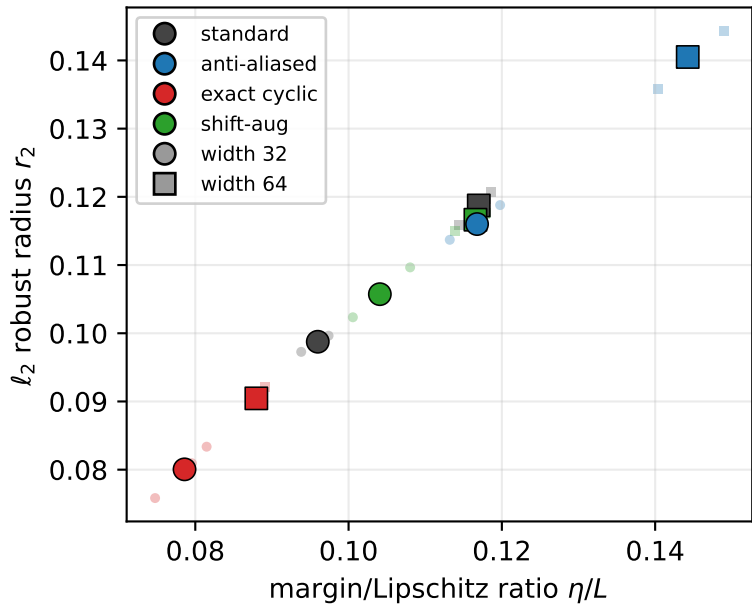
Pearson +1.00, Spearman +0.98
