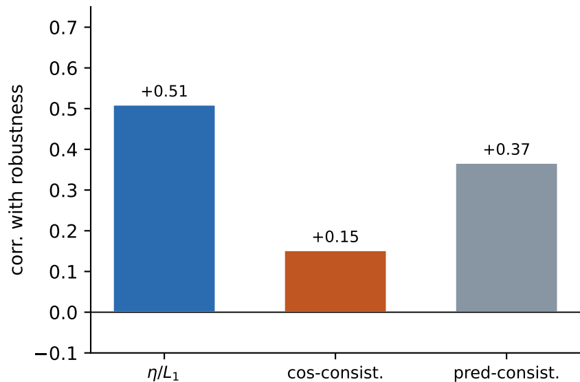
Controlling for adv. training
