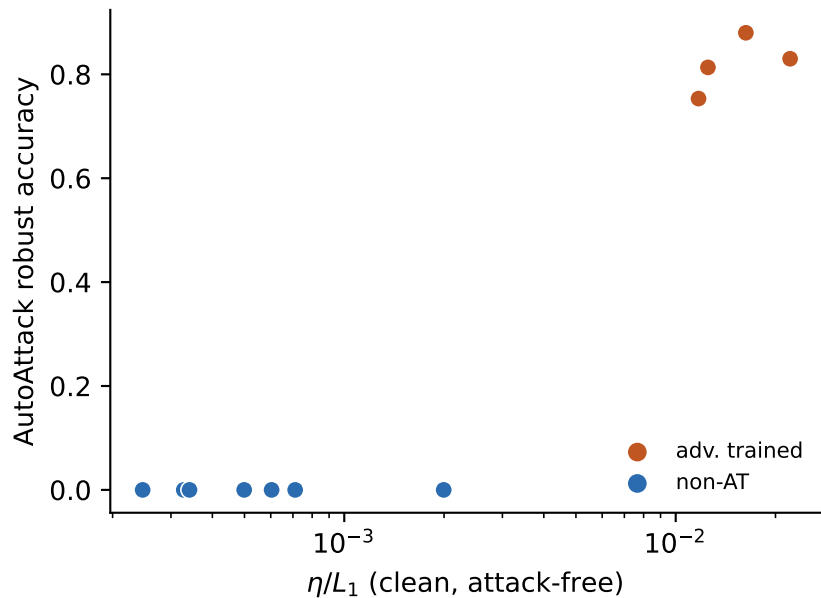
Tower ranking: Pearson = +0.95
