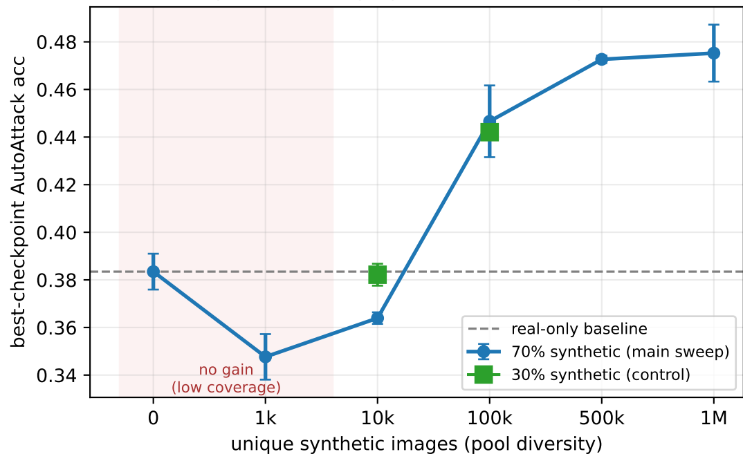
The gain is coverage-gated, not a mixing artifact
