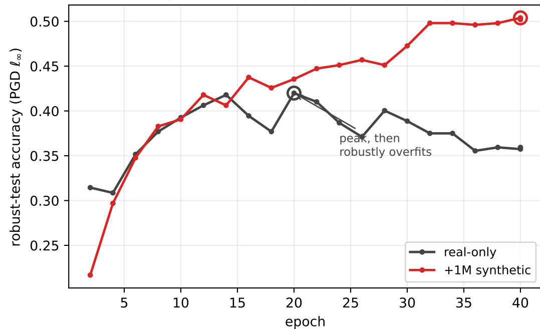
Synthetic data delays robust overfitting
