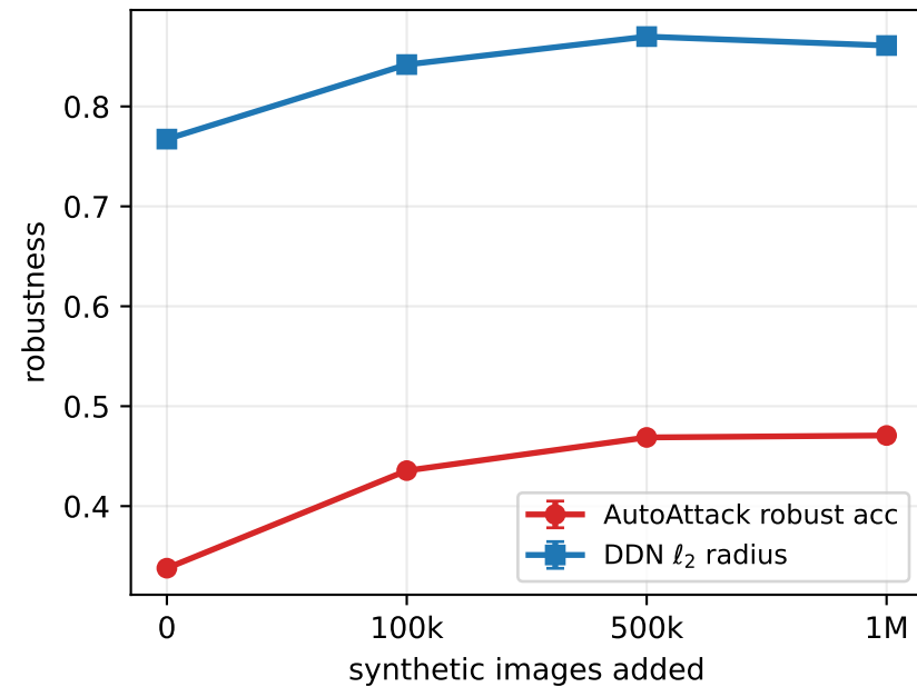
Robustness rises with synthetic data
