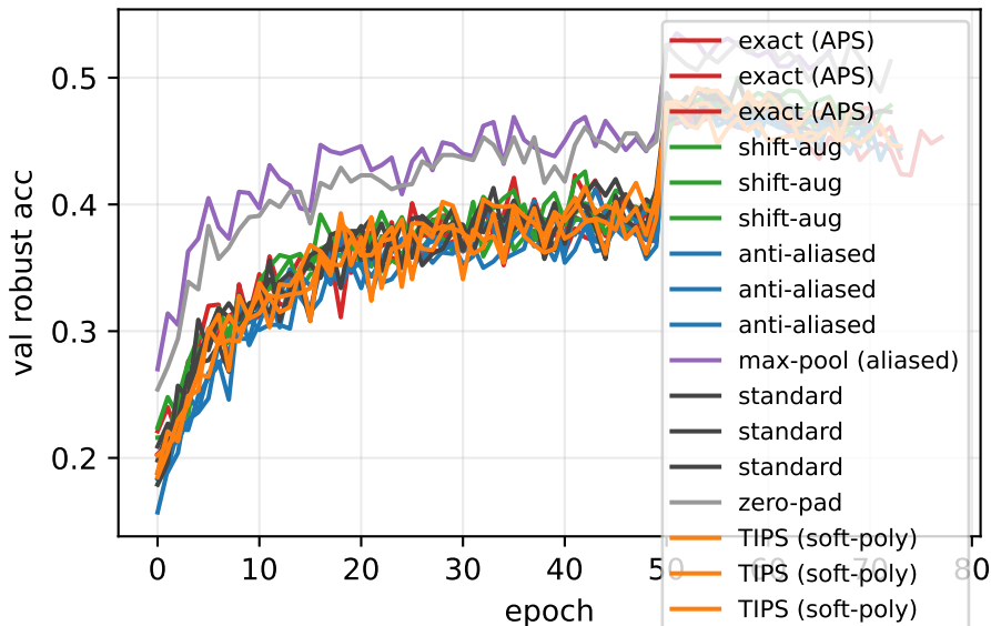
AT trajectories (robust overfitting)
