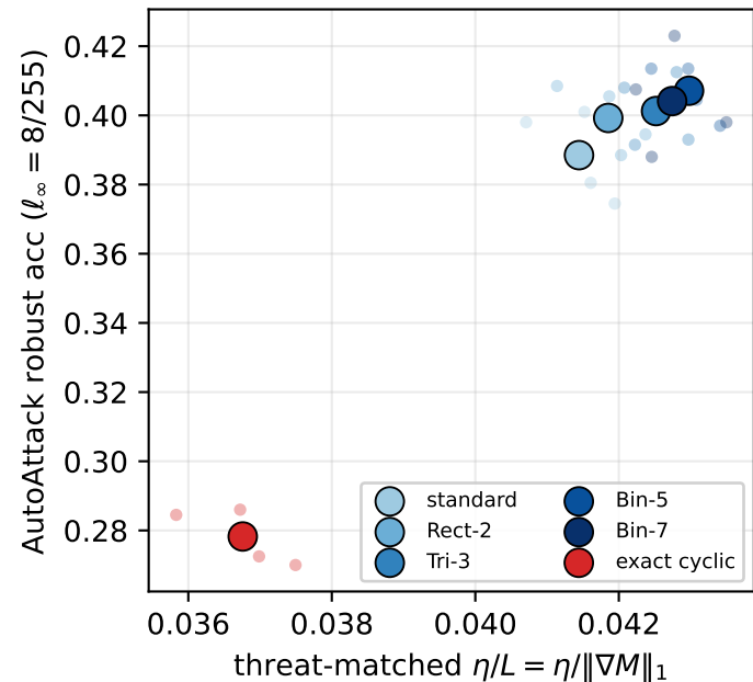
\eta/L tracks robustness (Pearson +0.93)
