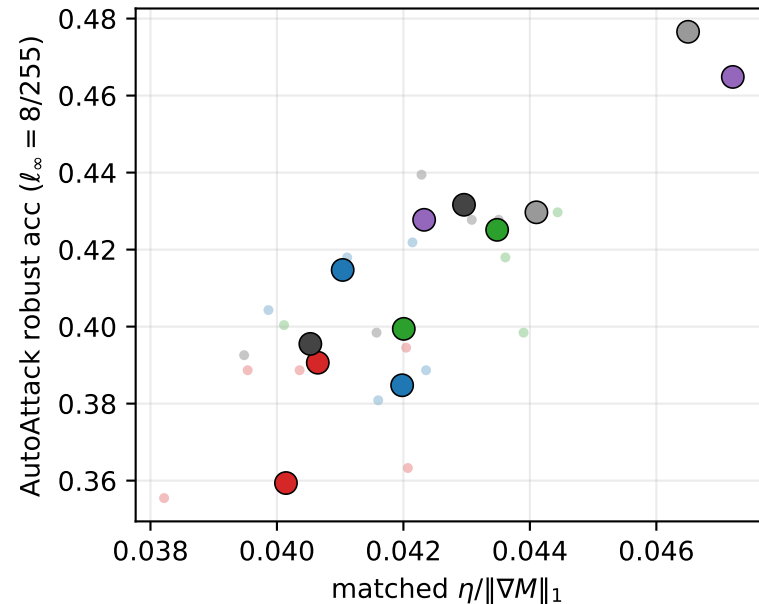
Pearson +0.90
