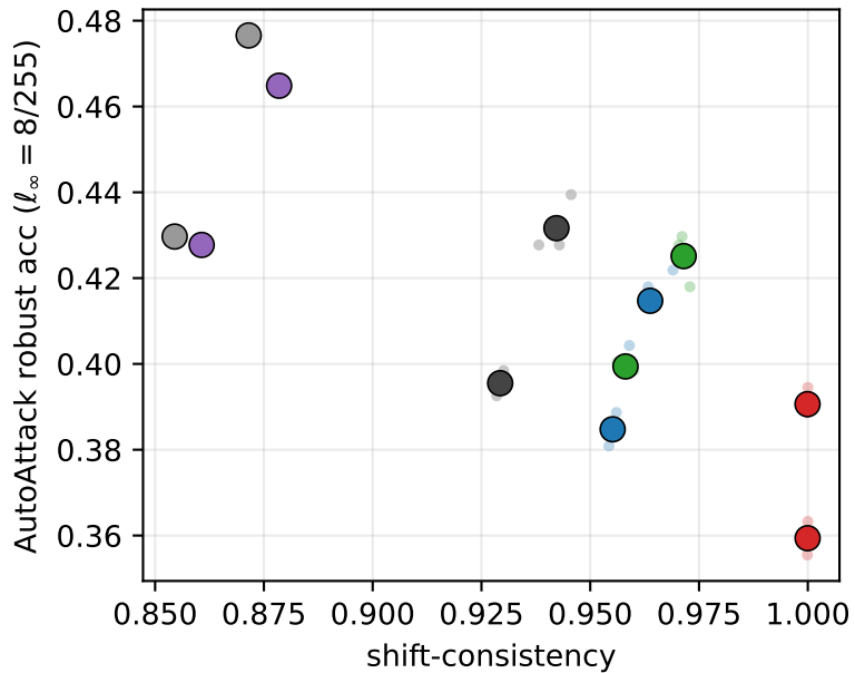
Pearson -0.74
