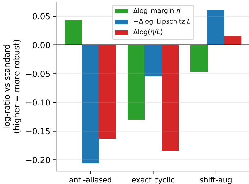
width 32 (AT)
