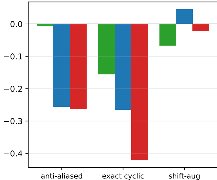
width 64 (AT)
