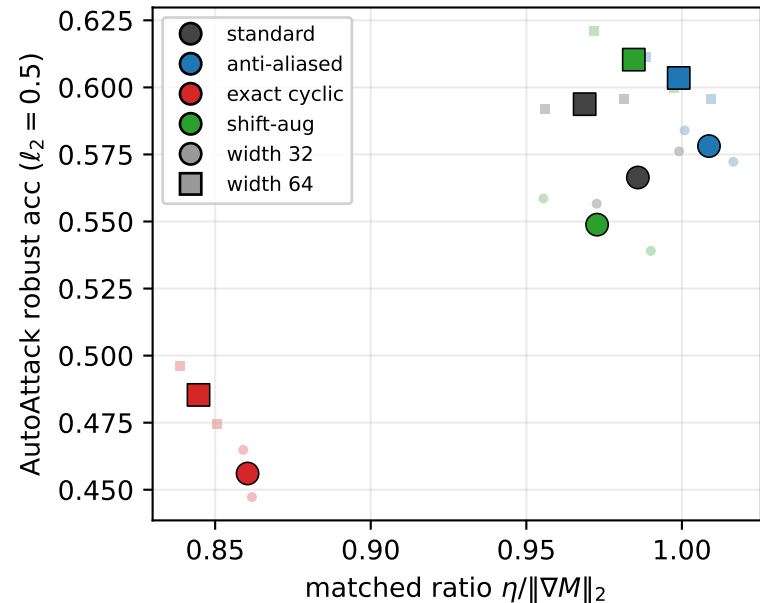
Pearson +0.91, Spearman +0.60
