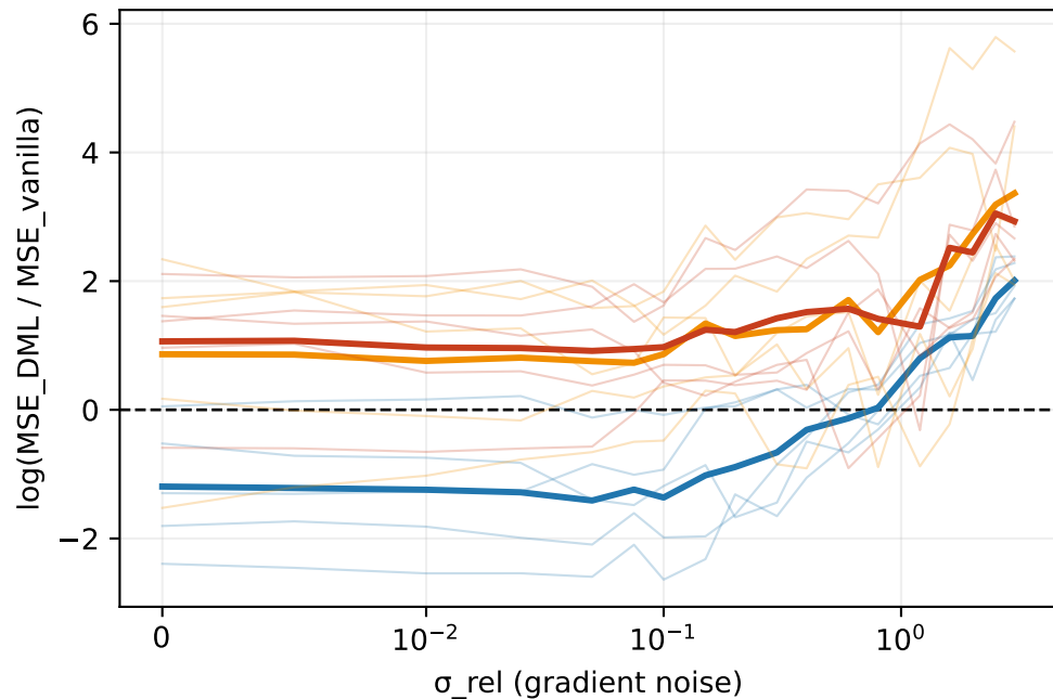
snake
