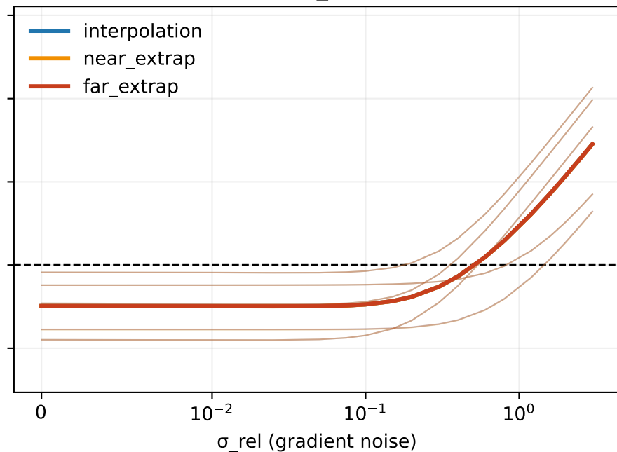
fourier_linear
