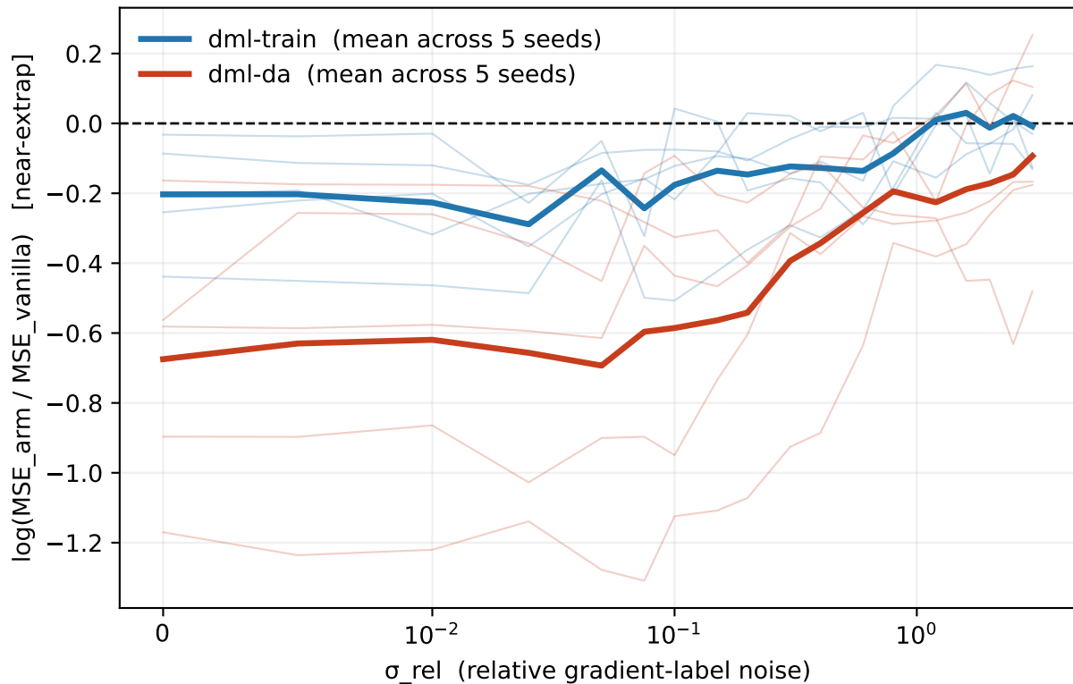
SIREN near-extrap — DA training improves \sigma^*
