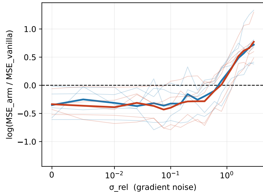
region = interpolation
