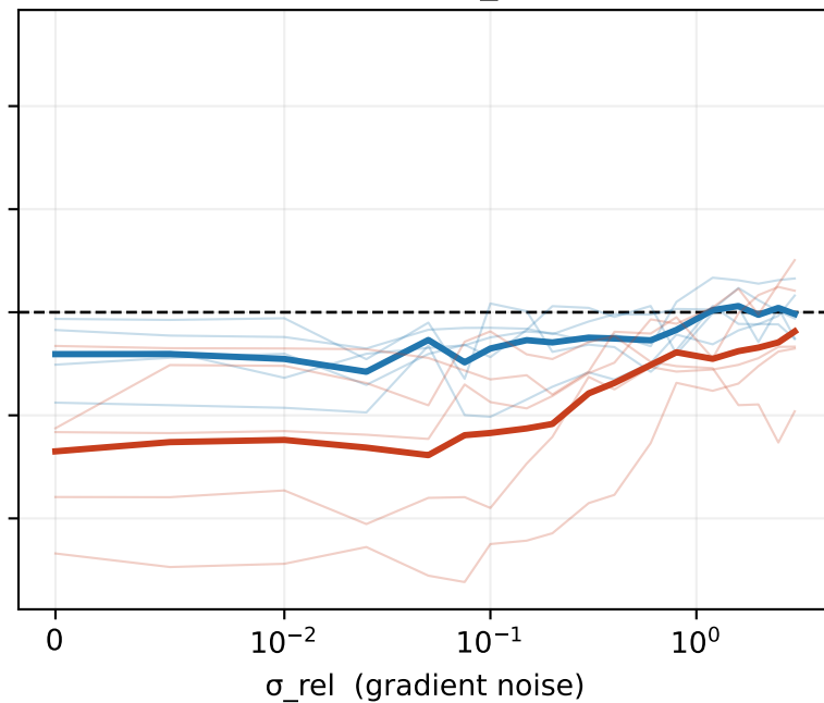
region = near_extrap
