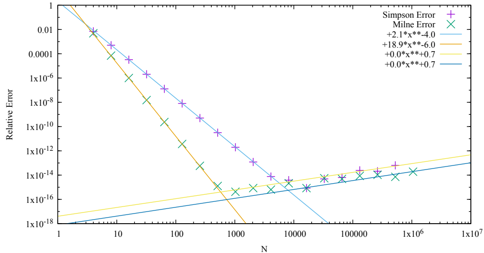
Relative Errors for Simpson/Milne Integration Routines
