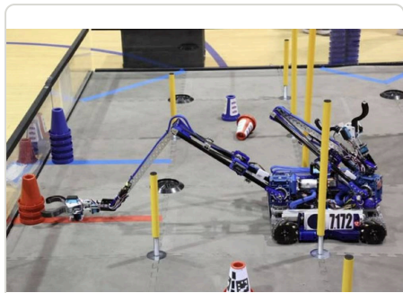
"Phoenix" (2022-23 Power Play) — dual-arm turret on extending drivetrain
