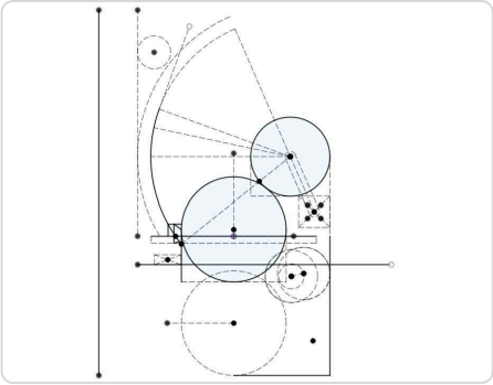
Shooter wheel geometry sketch
