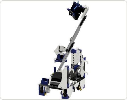
Passive two-way specimen claw — grabs and scores by driving
