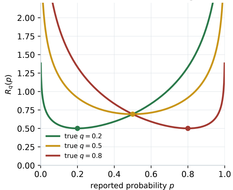
Truth minimizes expected log loss
