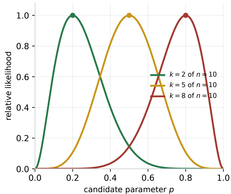
Data reshape the likelihood
