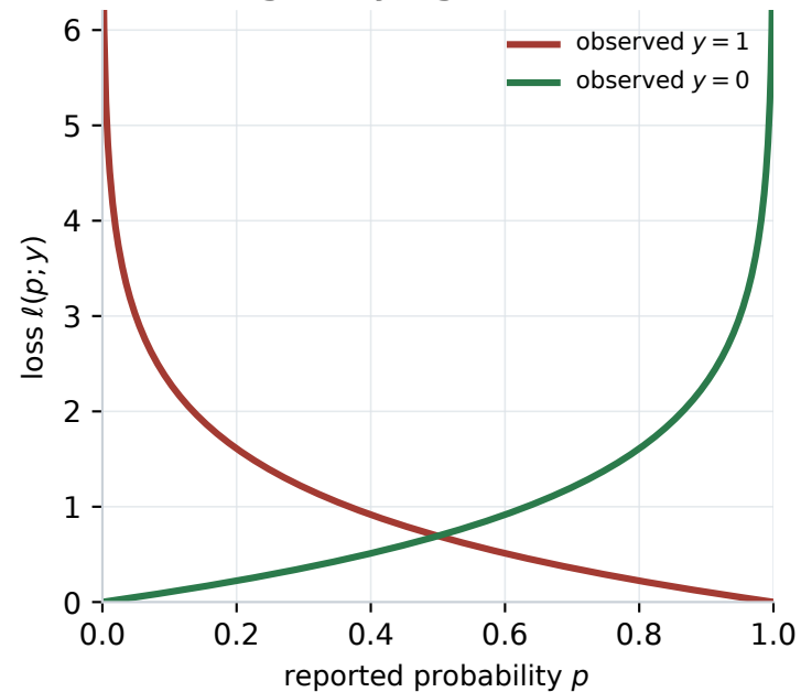
Log loss judges a report
